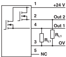
2 X PNP
